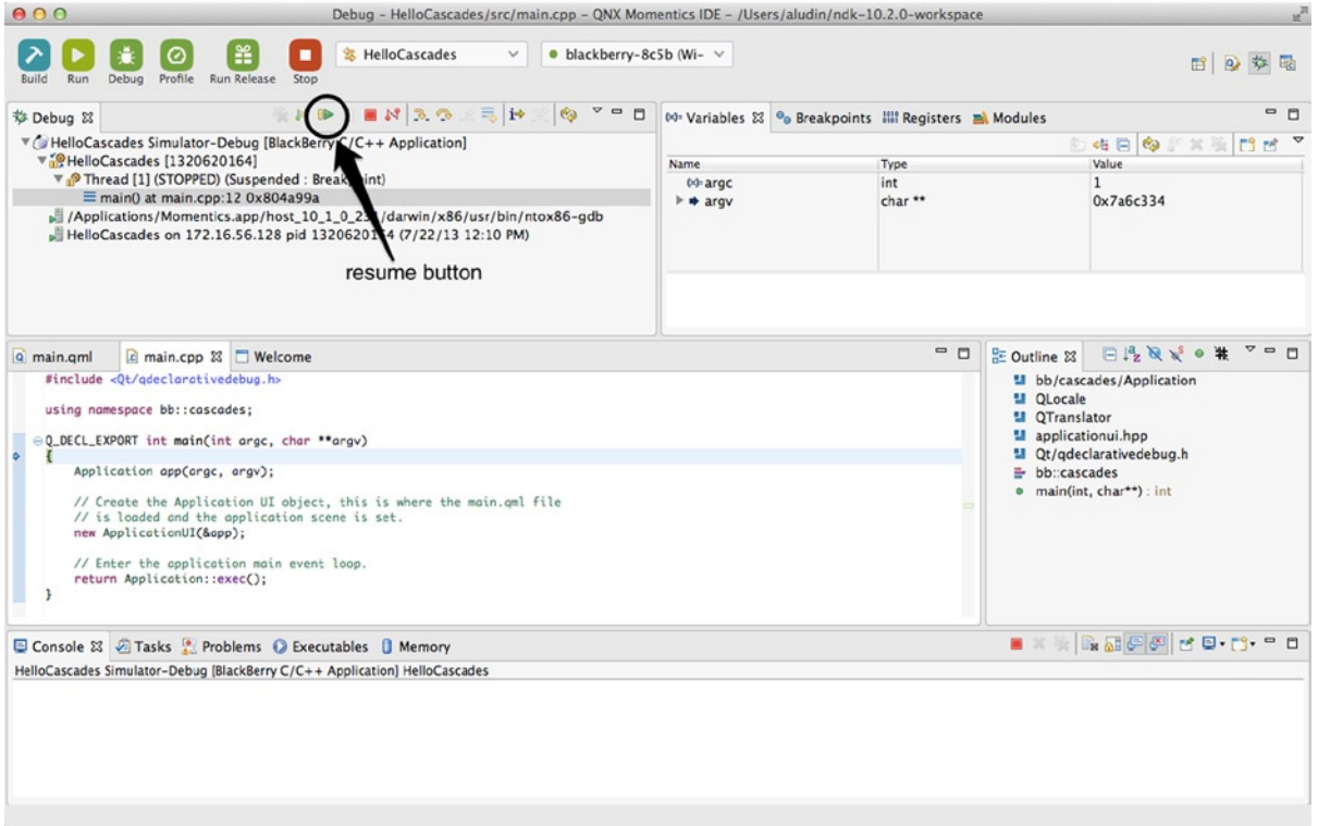
Figure 1-19. Debug perspective
